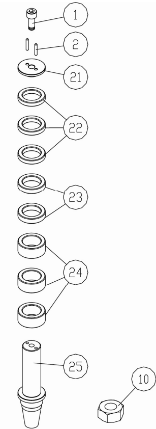
50mm Spindle
