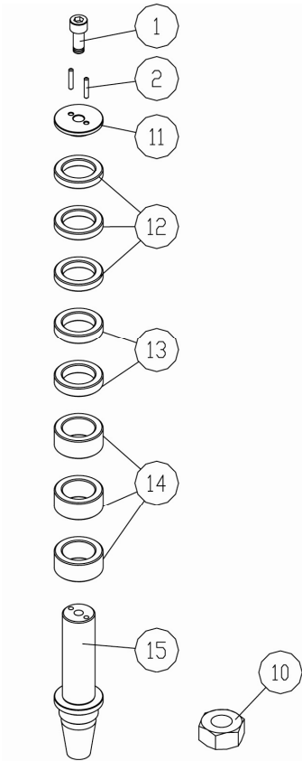
35mm Spindle
