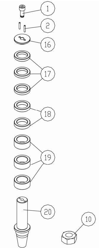
40mm Spindle
